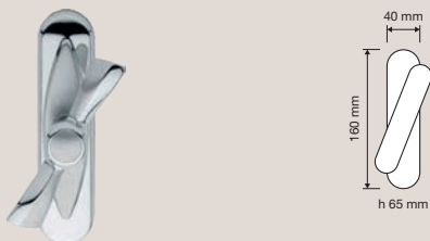
990 CR Cremonese / Window handle gratz
